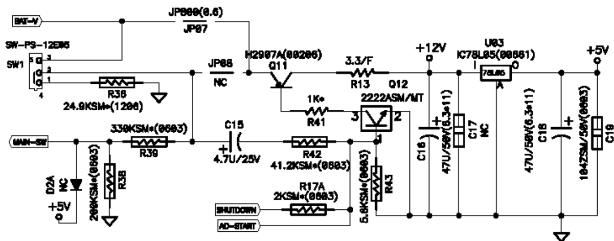
Figure S-2 Control Power Circuit
