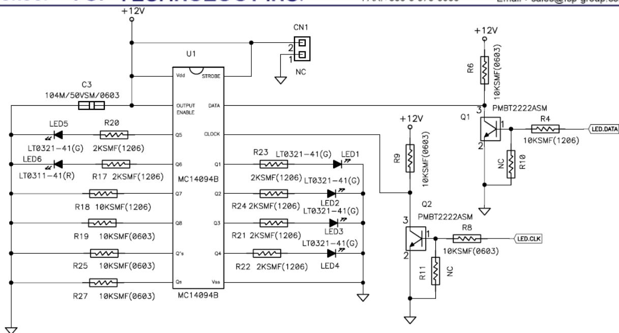
Figure S-8-B 6 LEDs Display Circuit
